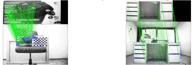
Fig. 3 Object recognition using SIFT features. Left image shows a carton being recognized, right image shows a table being recognized. Objects used in this work include cartons of different kinds, a table, a chair, a shelf & a mug.
